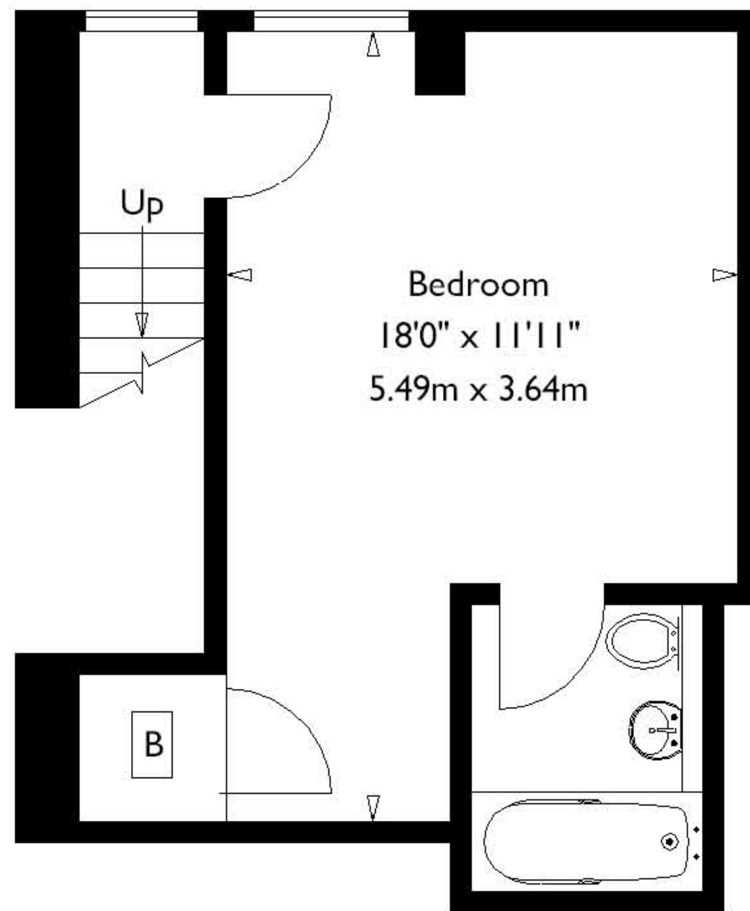
Lower Ground Floor
