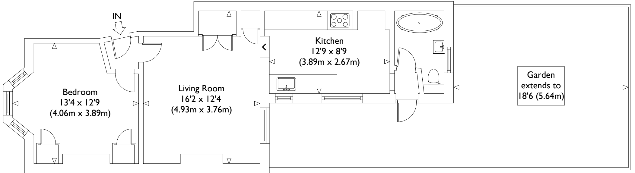
Ground Floor
