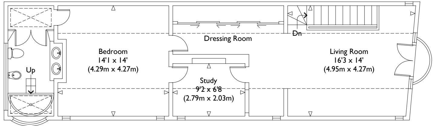
First Floor
