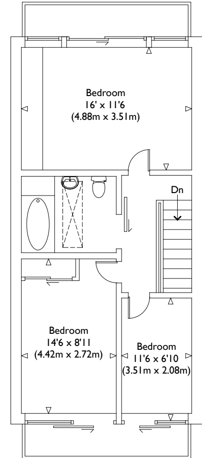
Second Floor
