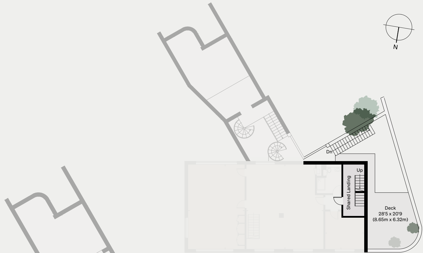
FIRST FLOOR
