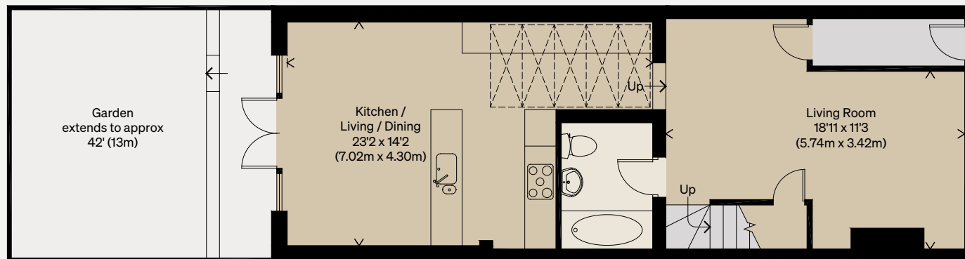
Ground Floor
