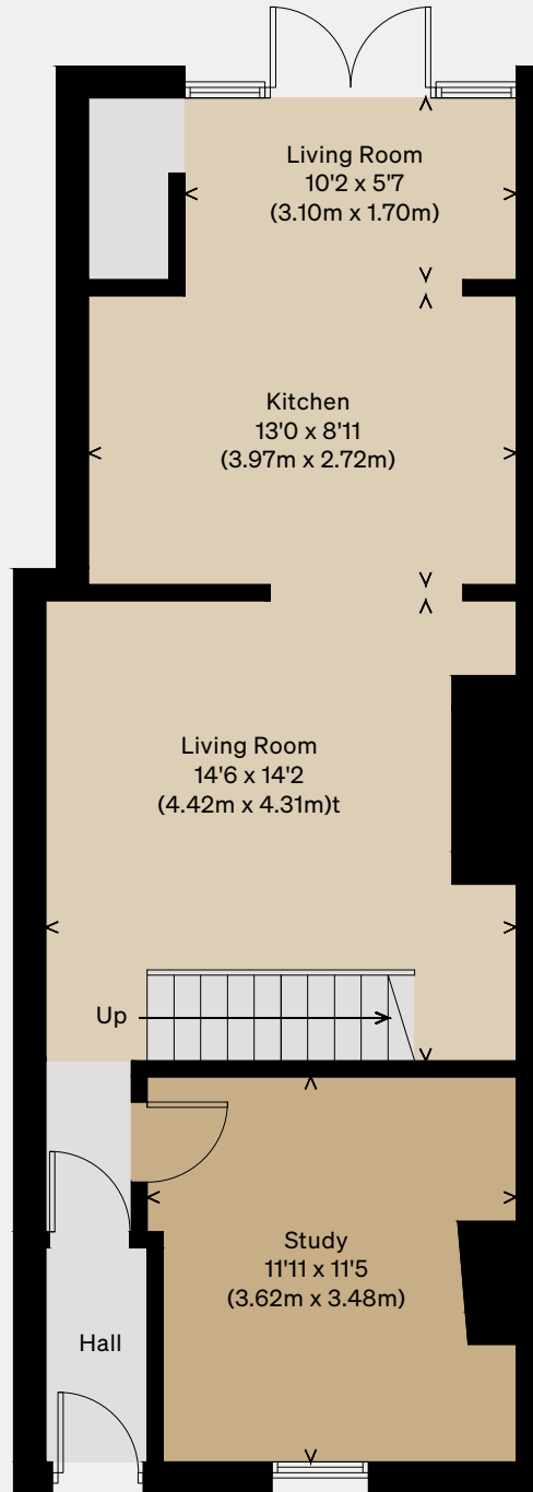
GROUND FLOOR
