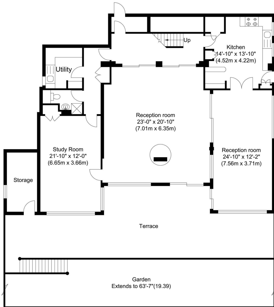
Ground Floor Approximate Floor Area 1765.29 sq. ft. (164 sq. m)
