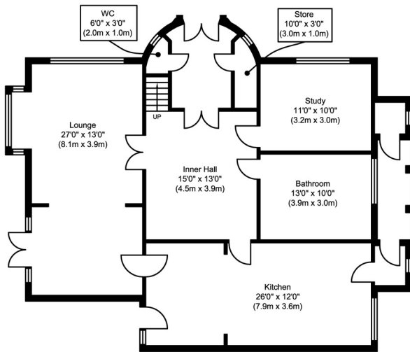
Ground Floor Approximate Floor Area 1379.07 sq. ft. (128.12 sq. m)
