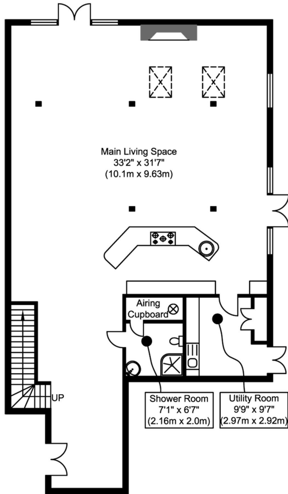
Ground Floor Approximate Floor Area 1472 sq. ft. (136.7 sq. m)
