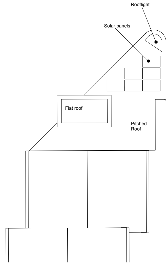
Roof plan 1:100
