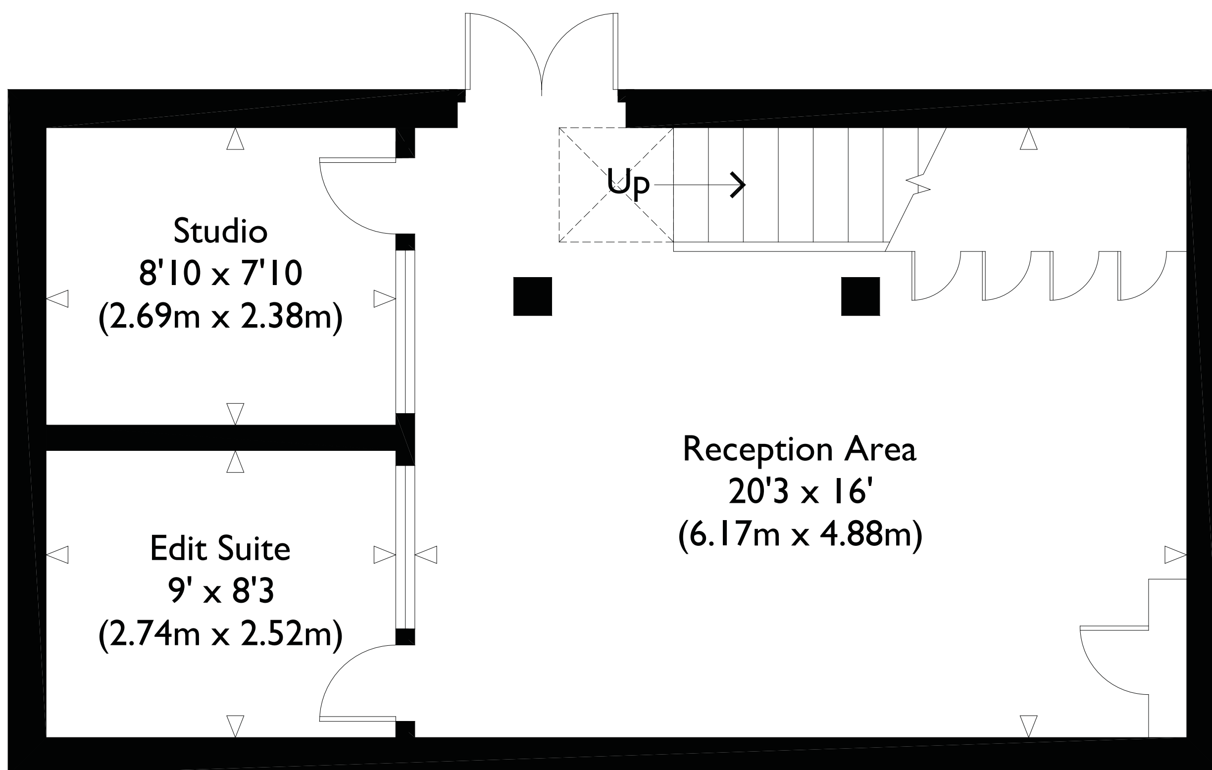
Ground Floor
